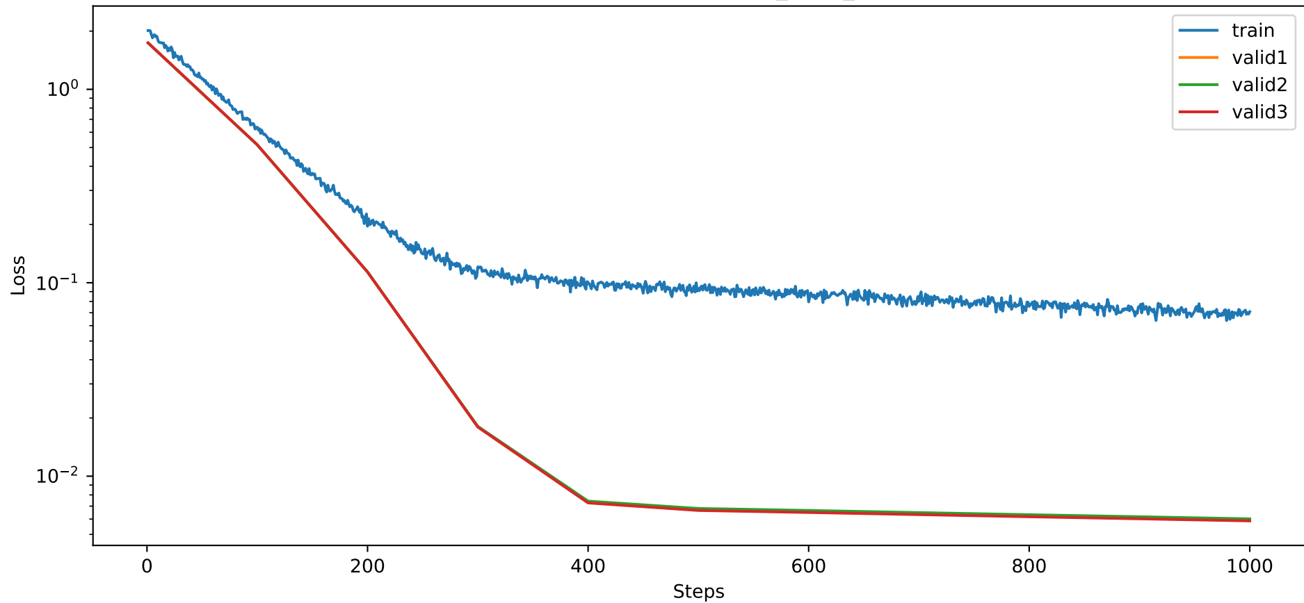
Training NMSE of PatchTST_revin_NMSE
