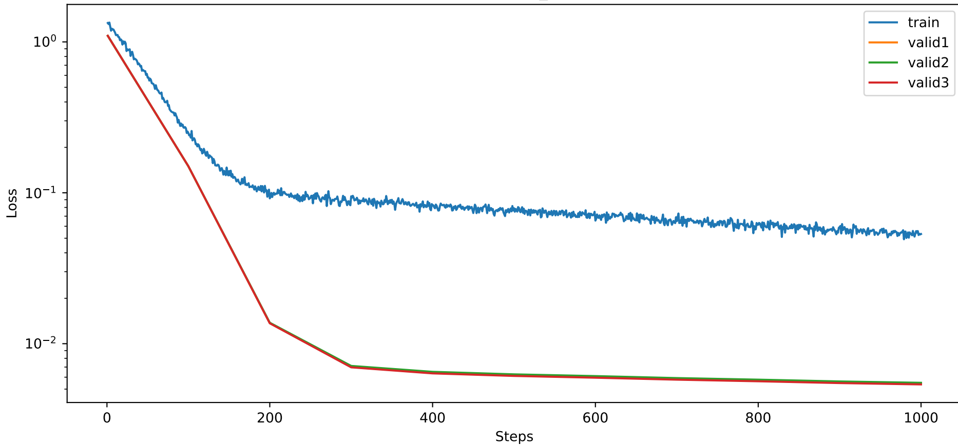
Training NMSE of min_fixed+gamma
