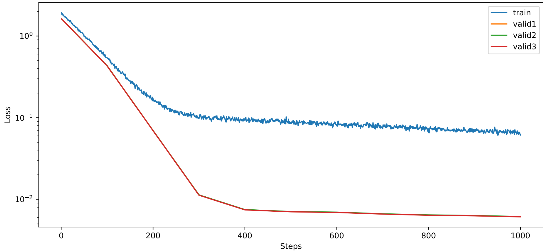
Training NMSE of min+revin
