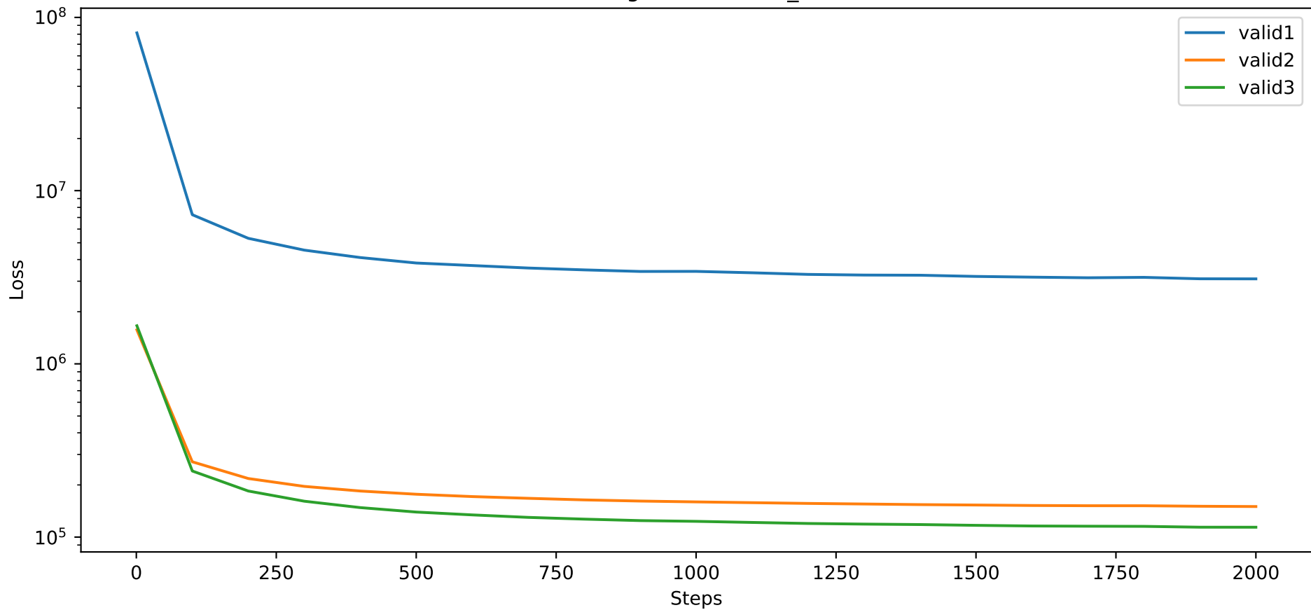
Training MSE of revin_min
