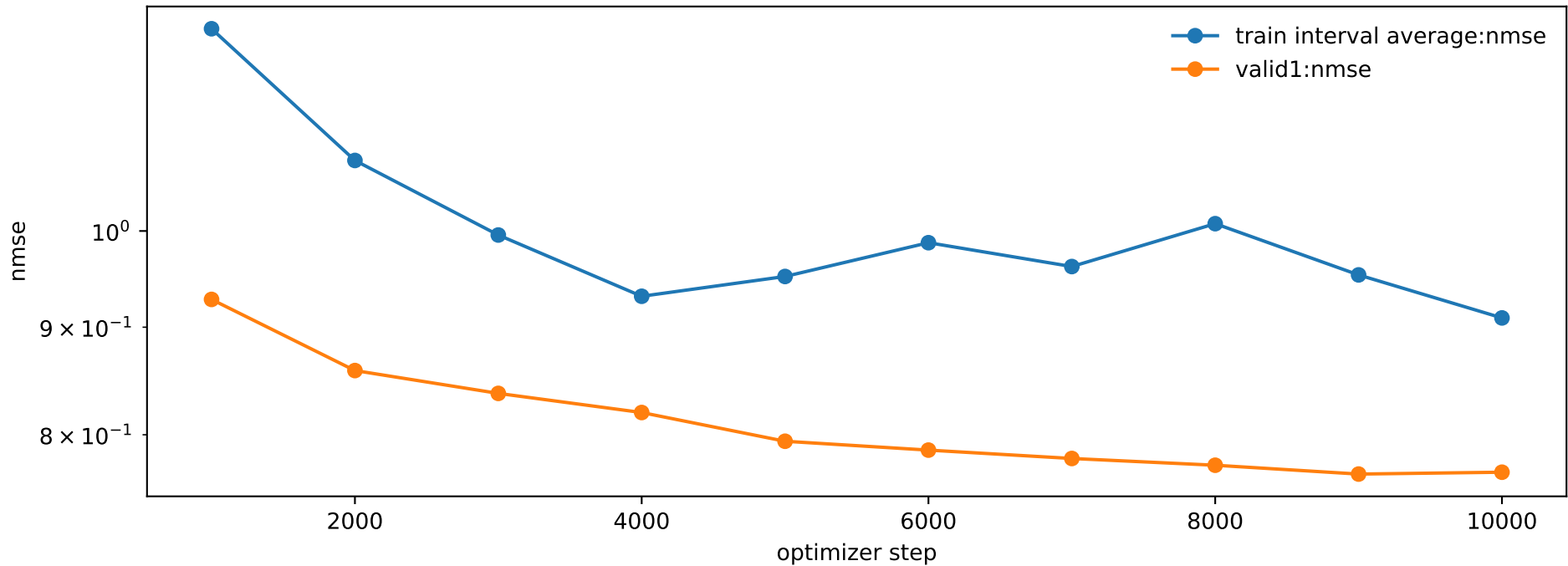
Criterion loss
