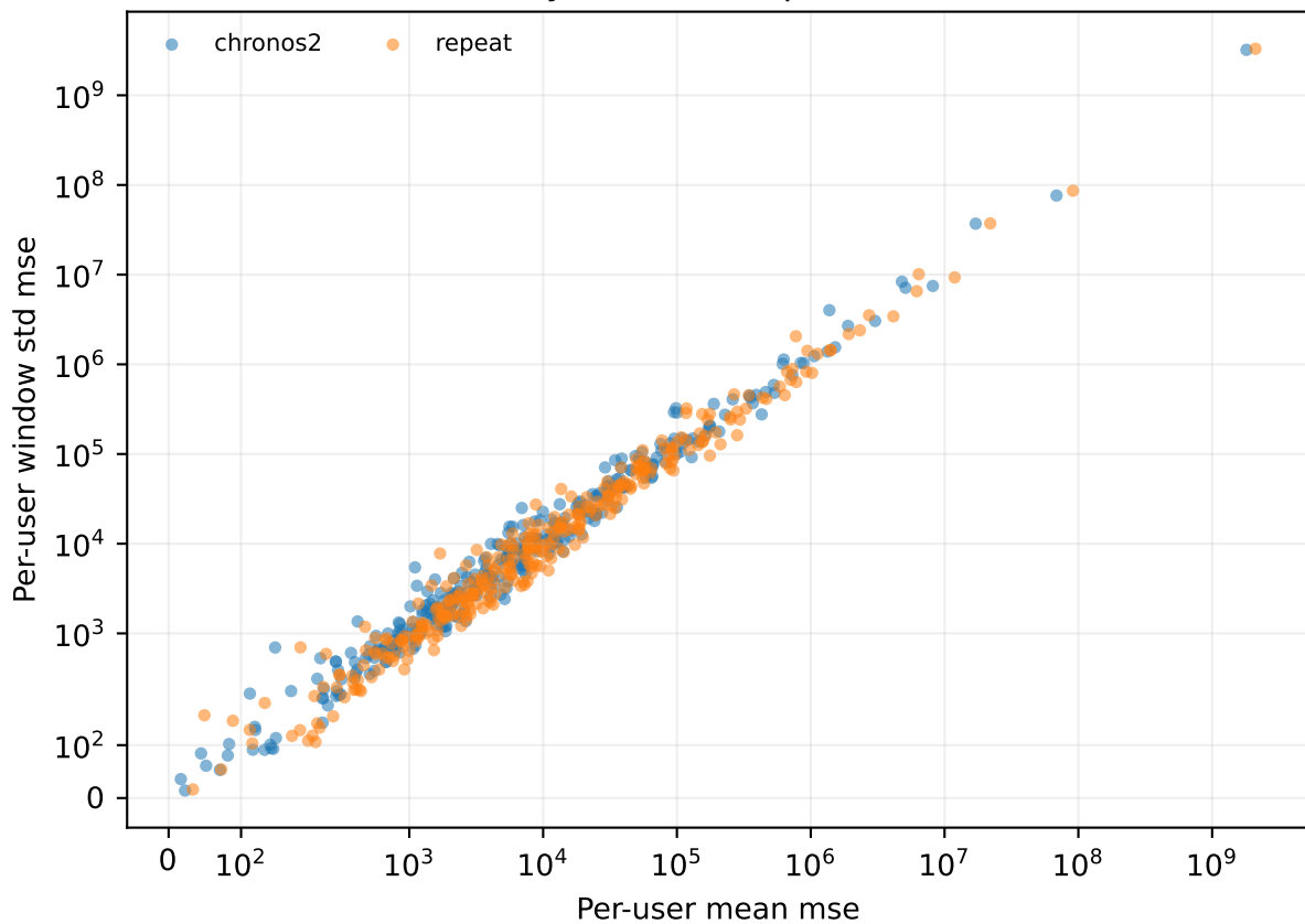
electricity 504:168 — per-user errors
