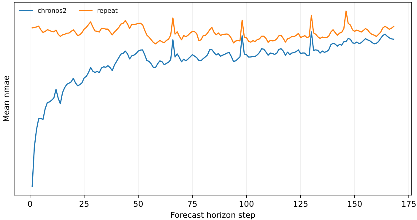
electricity 504:168 — horizon errors
