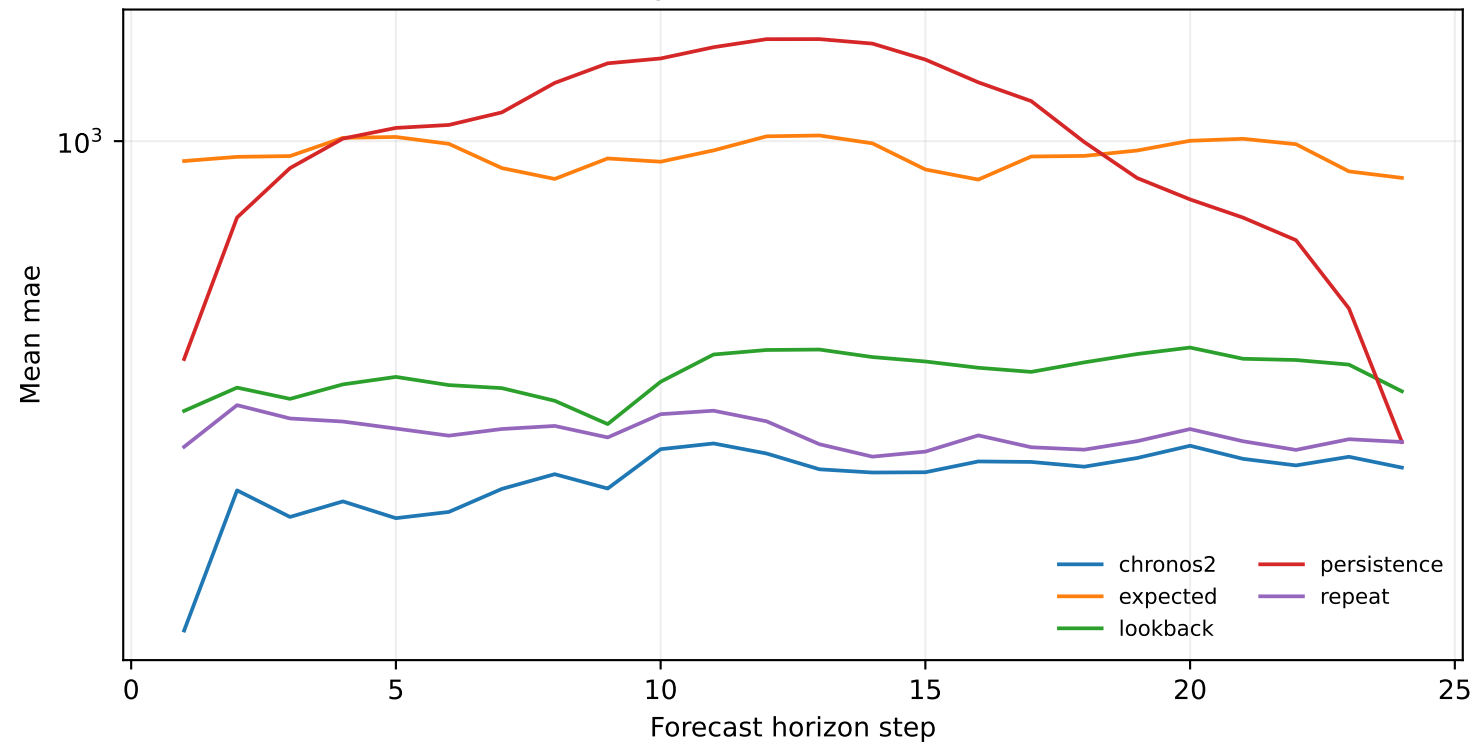
electricity 168:24 — horizon errors
