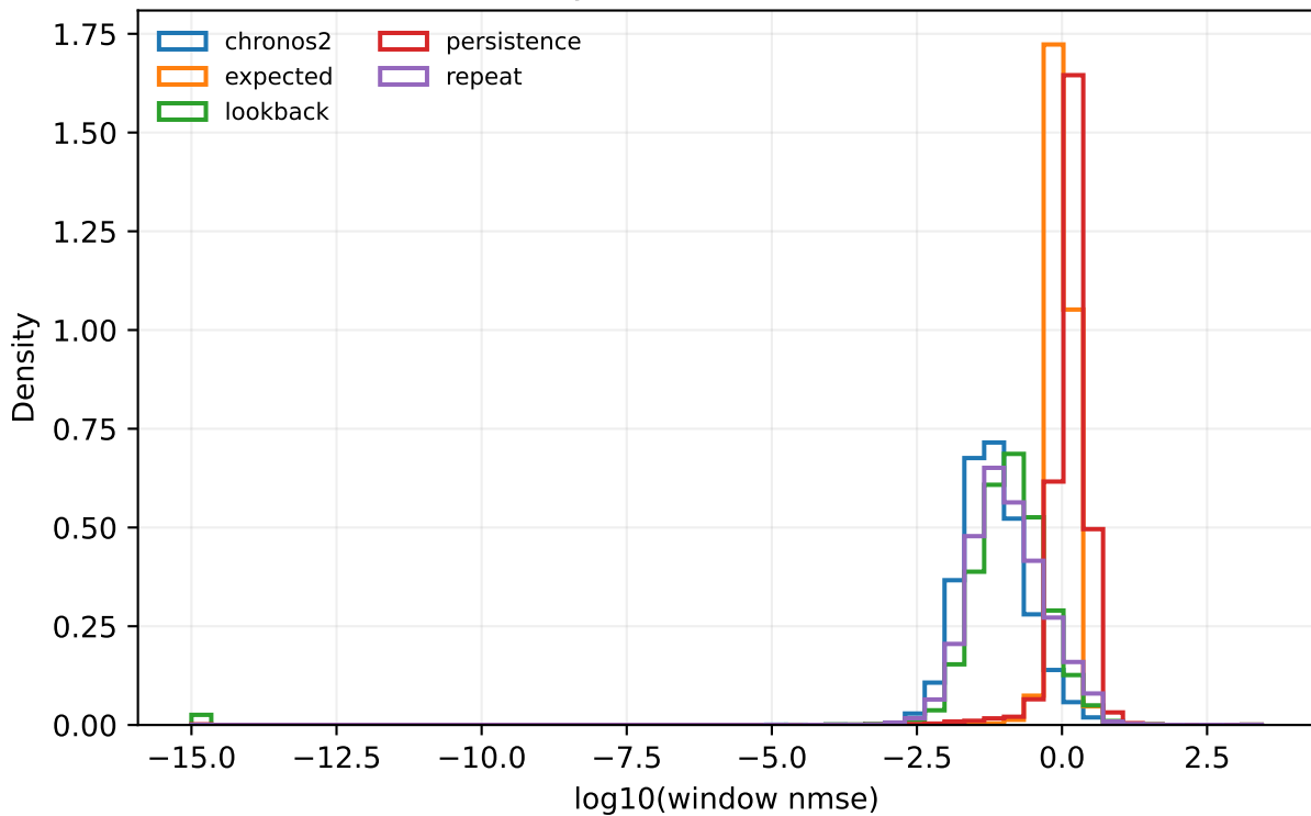
electricity 168:24 — window errors
