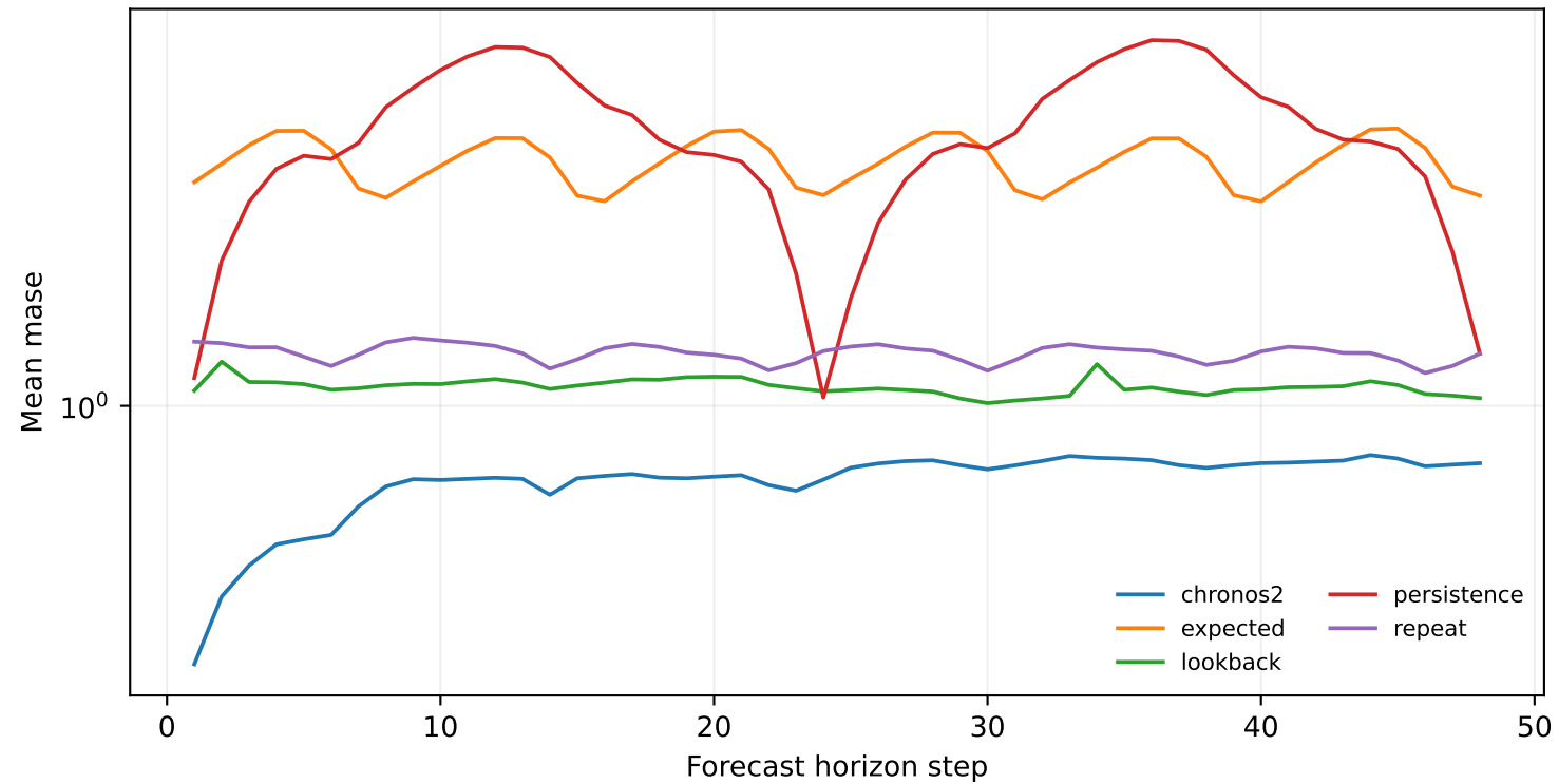
electricity 336:48 — horizon errors
