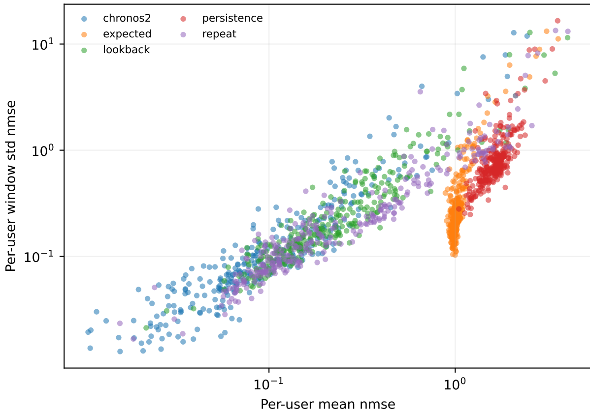
electricity 336:48 — per-user errors
