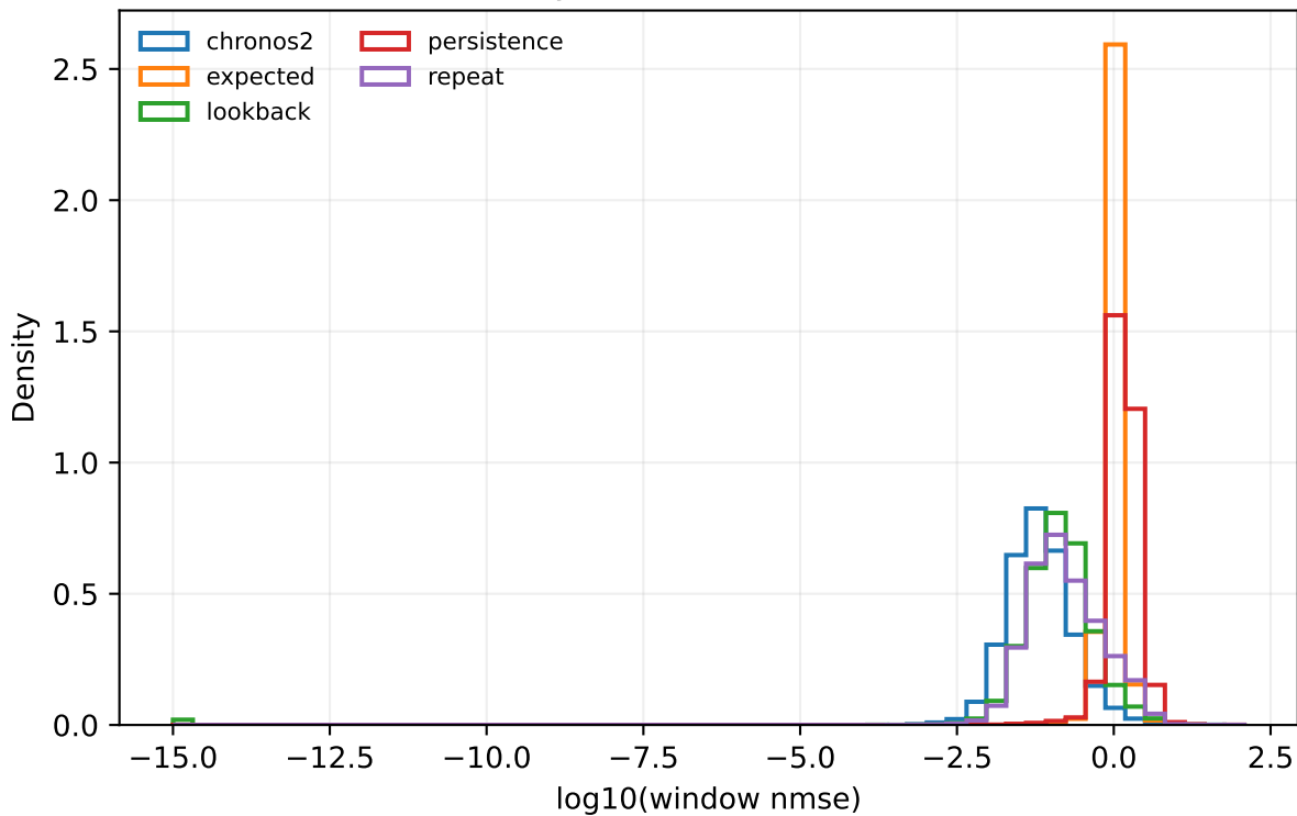
electricity 336:48 — window errors
