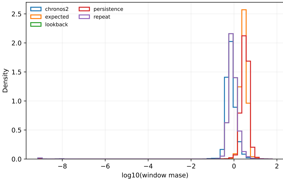
electricity 504:168 — window errors
