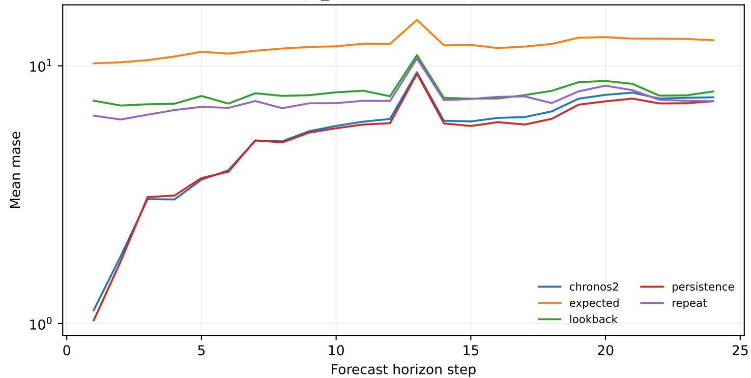
exchange_rate 168:24 — horizon errors
