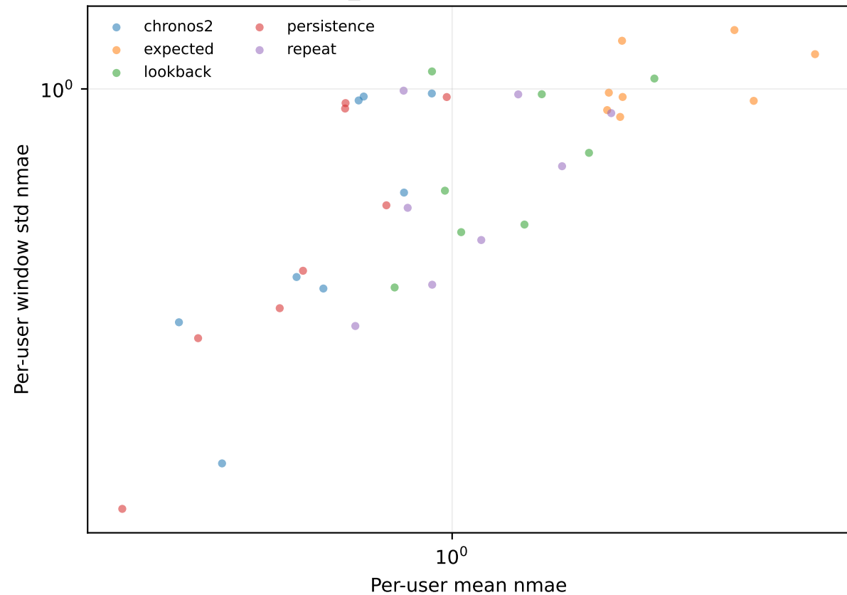
exchange_rate 168:24 — per-user errors
