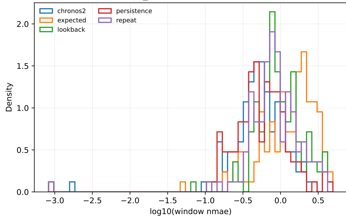
exchange_rate 168:24 — window errors
