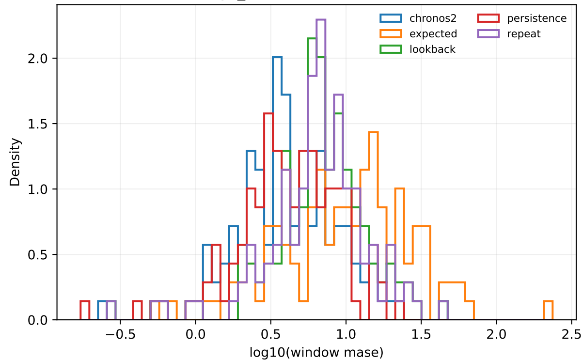
exchange_rate 336:48 — window errors
