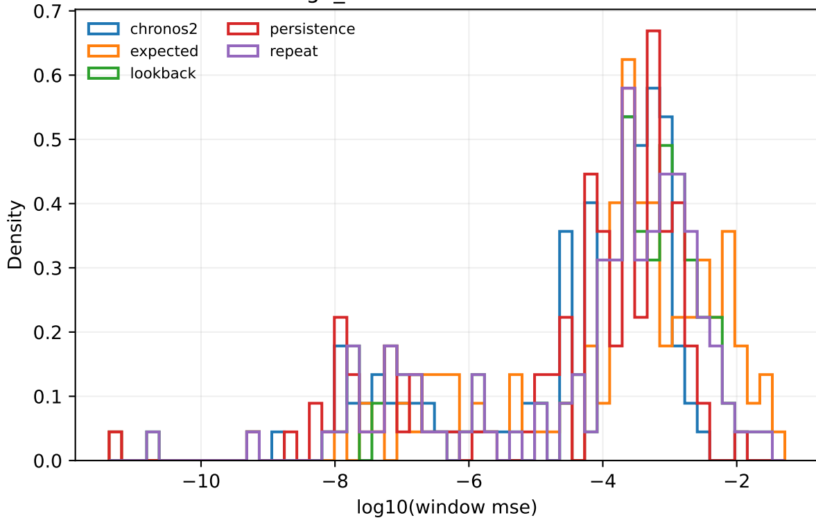
exchange_rate 336:48 — window errors
