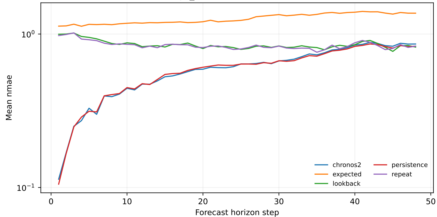
exchange_rate 336:48 — horizon errors
