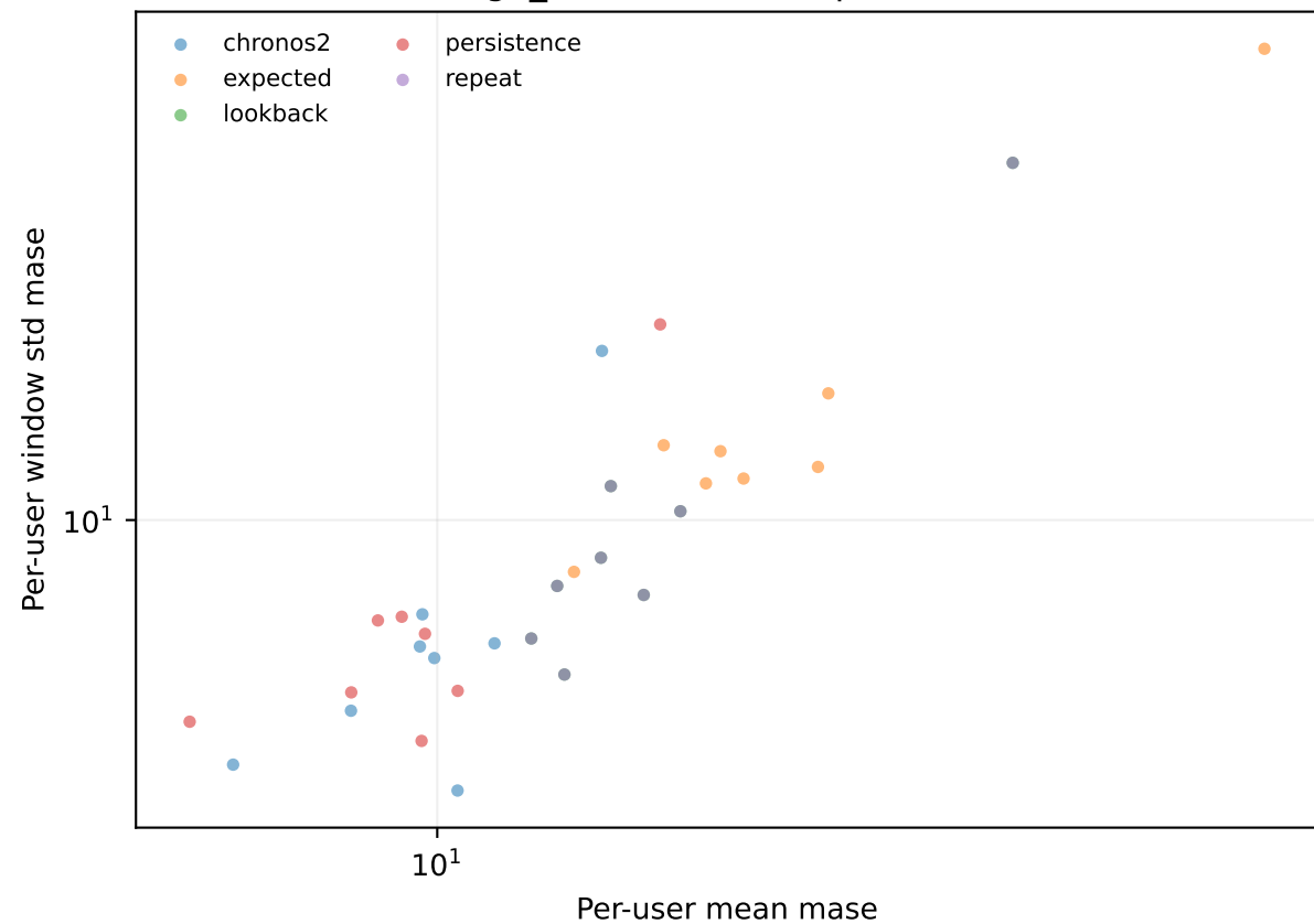
exchange_rate 504:168 — per-user errors
