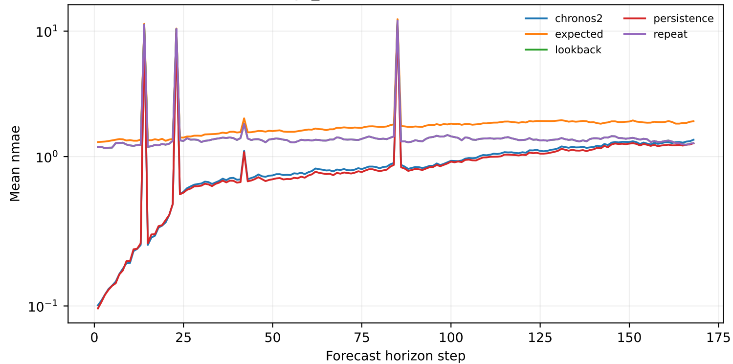
exchange_rate 504:168 — horizon errors
