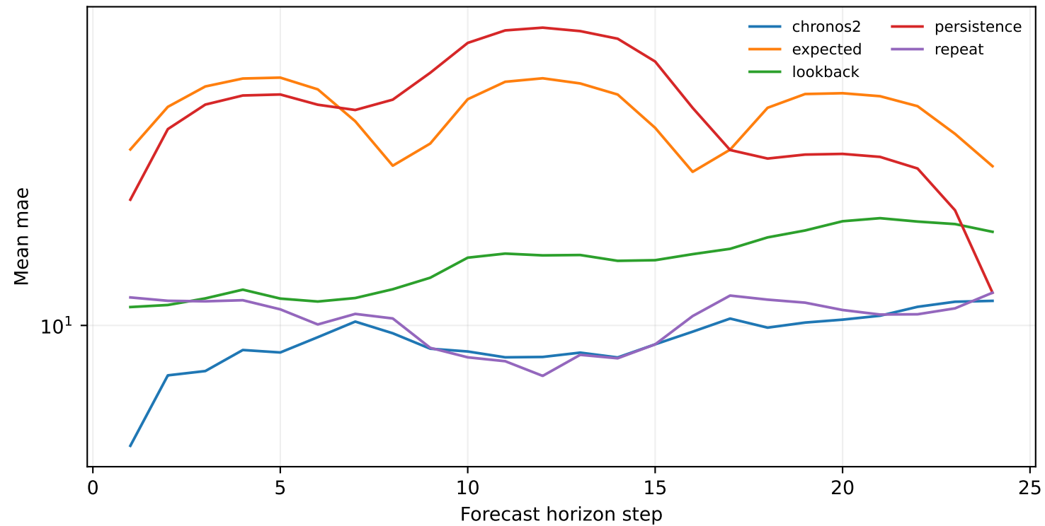
solar 168:24 — horizon errors
