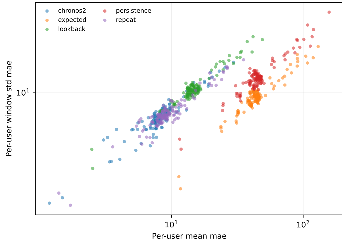
solar 168:24 — per-user errors
