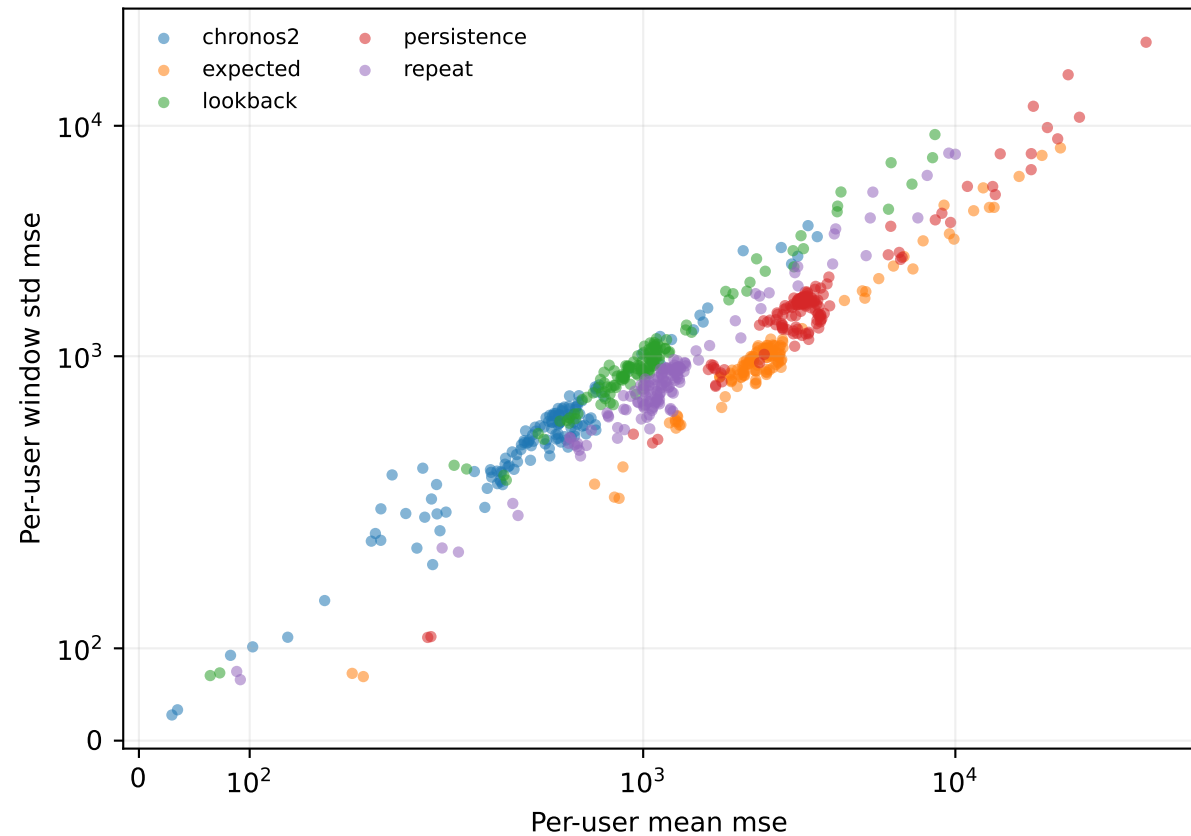
solar 336:48 — per-user errors
