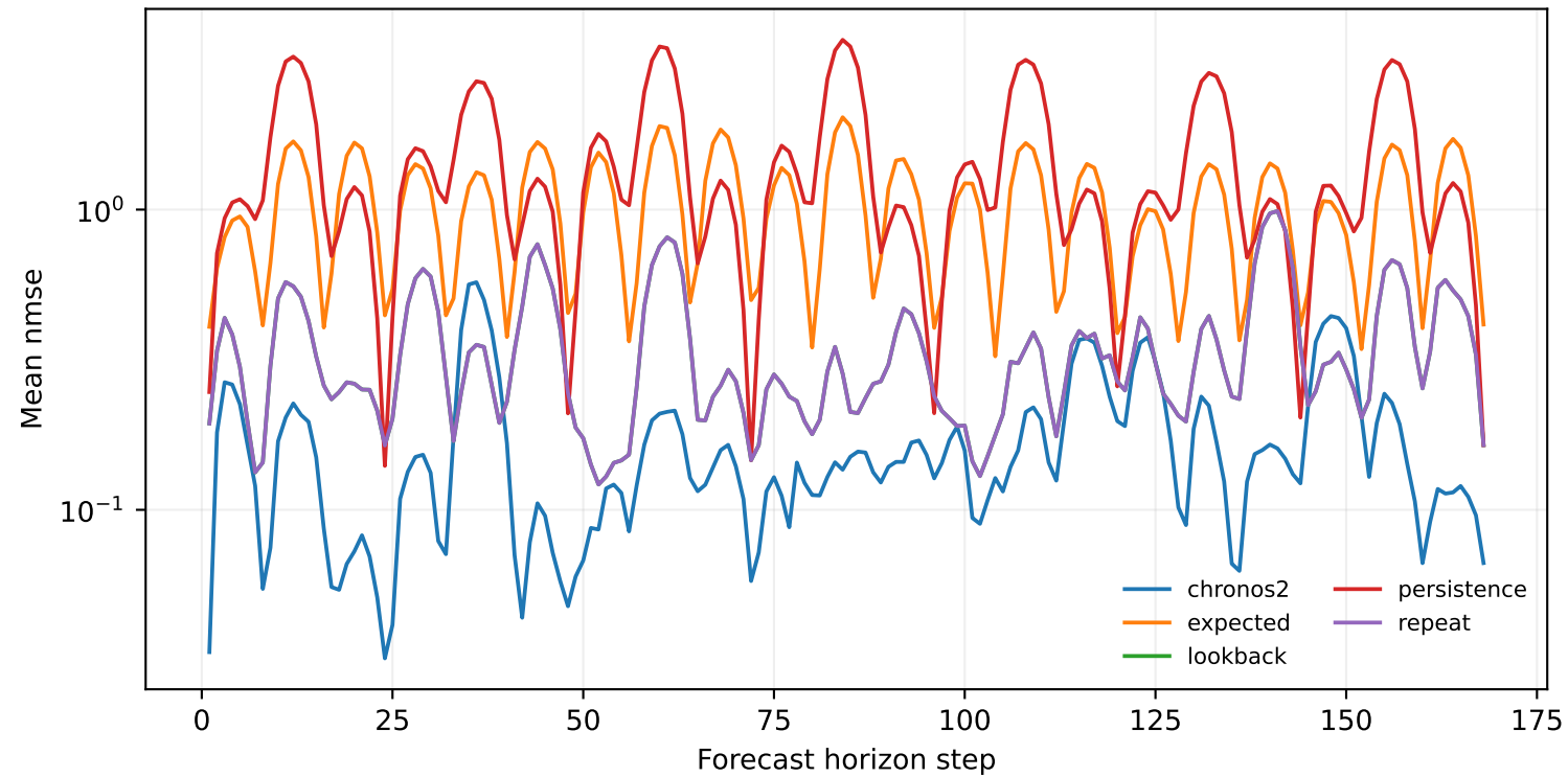
solar 504:168 — horizon errors
