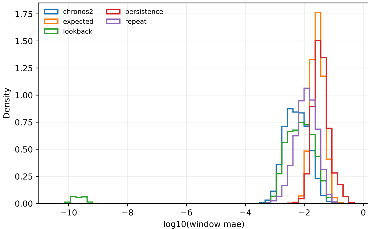
traffic 168:24 — window errors
