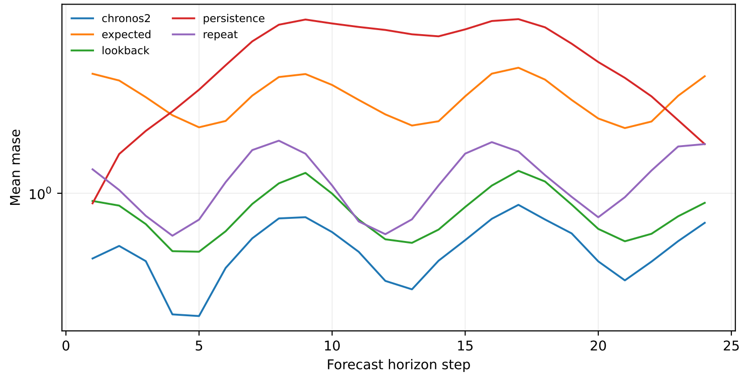
traffic 168:24 — horizon errors
