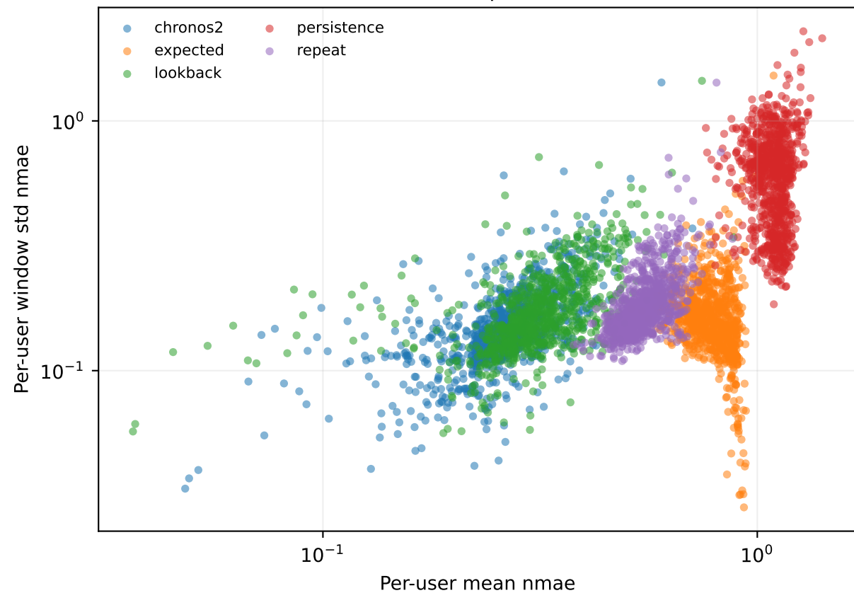
traffic 336:48 — per-user errors
