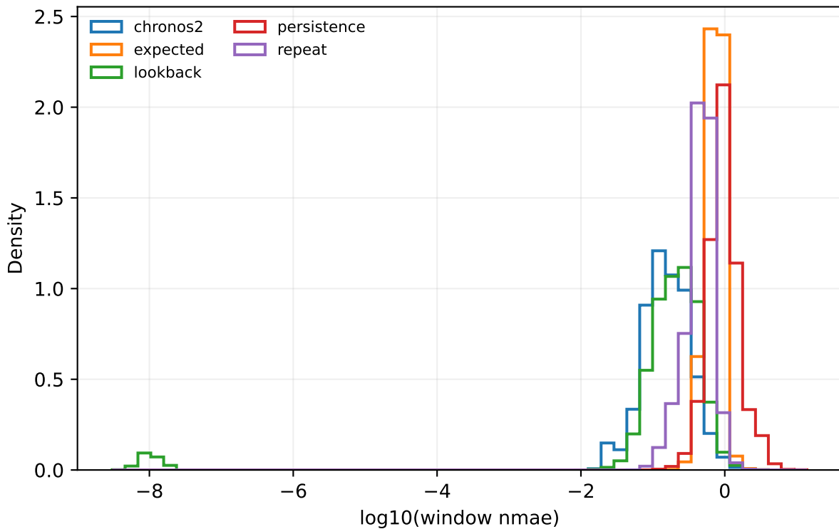
traffic 336:48 — window errors
