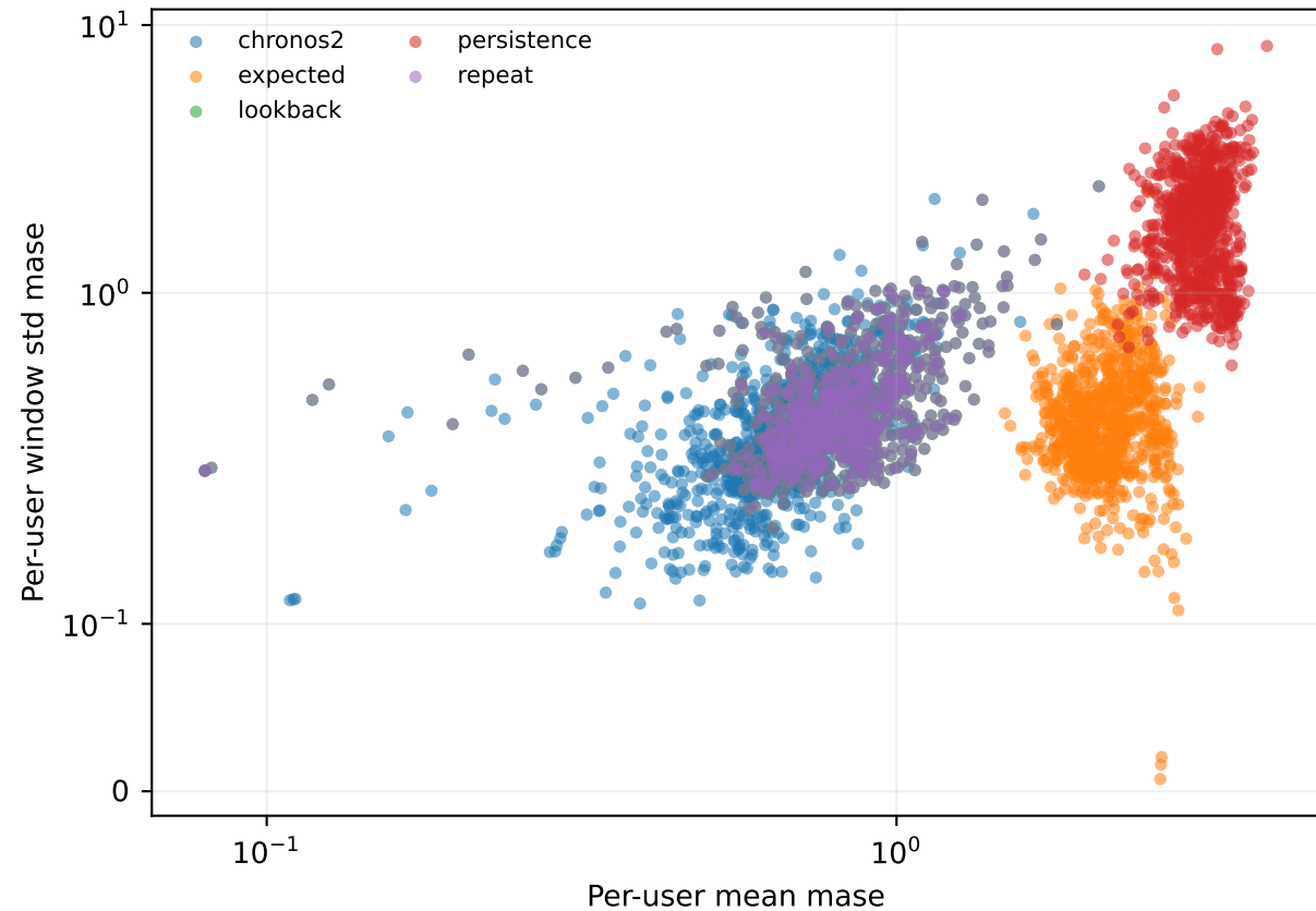
traffic 504:168 — per-user errors
