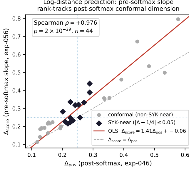
Figure 1: The log-distance prediction, tested head-by-head (exp-056). Scatter: pre-softmax slope \Delta_{\text{score}} vs. post-softmax conformal dimension \Delta_{\text{pos}} for the 44 conformal GPT-2 heads (grey: non-SYK-near; diamonds: SYK-near heads, |\Delta - 1/4| \leq 0.05 ). Red line: OLS regression. Dotted: identity \Delta_{\text{score}} = \Delta_{\text{pos}} . The raw query-key computation encodes the conformal dimension rank-for-rank at Spearman \rho = +0.976 . The OLS slope ( \approx 1.4 ) reflects the softmax renormalization discussed in the text.
