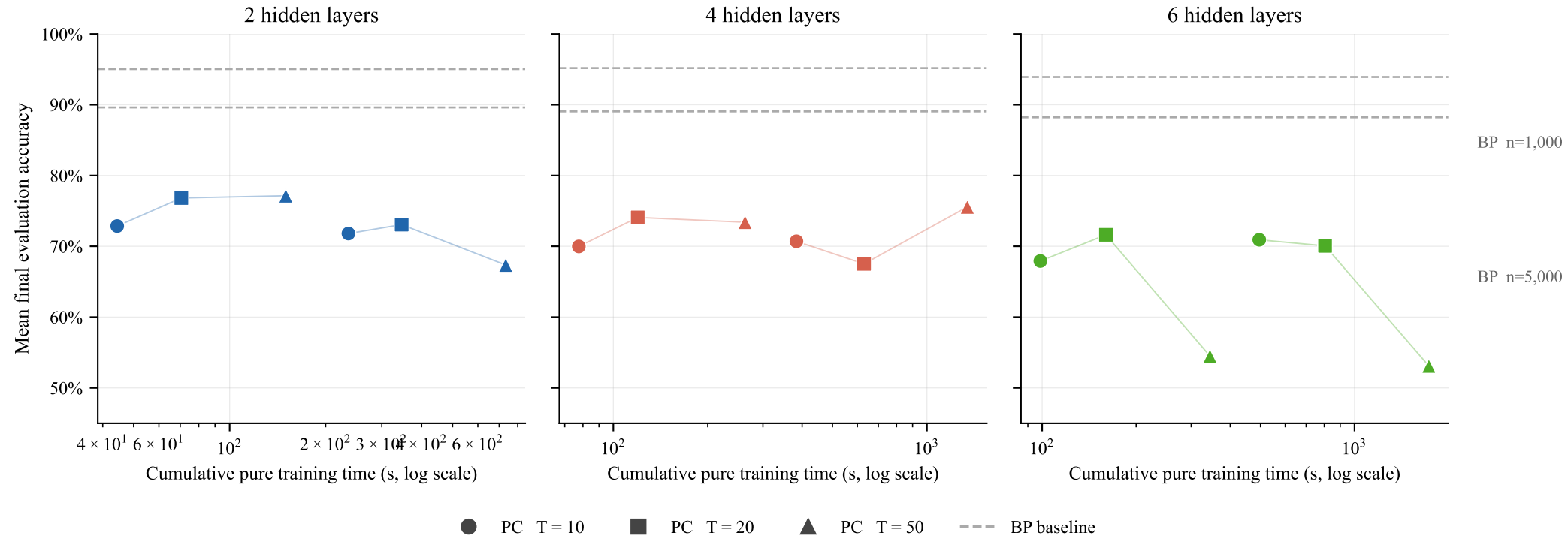
Figure 1. Accuracy–compute trade-off map for the confirmatory grid Each marker = one (depth, training size, T) configuration, mean across 5 seeds. Dashed lines = matched BP baselines.
