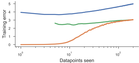
HMM - training
