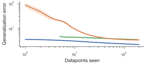
HMM - generalization
