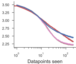
HMM
