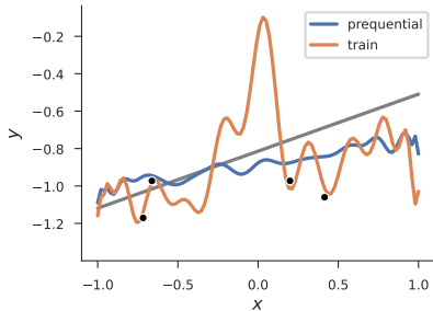
Datapoints seen = 4
