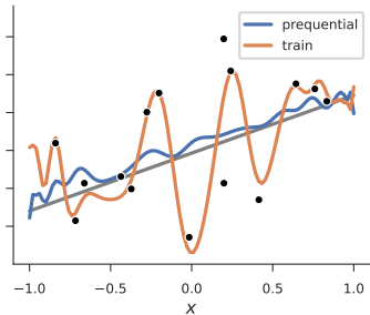
Datapoints seen = 15
