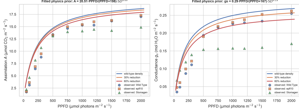
Fig. 7 Fitted physics priors (Eq. 3) for assimilation (left) and conductance (right) at three stomatal densities, overlaid on the Karavolias et al. (2023) light-response measurements.
