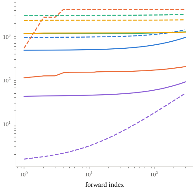
tiny-gpt2
