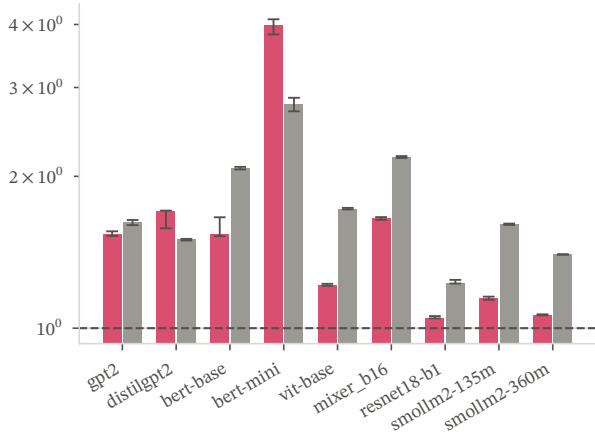
latency relative to the DAG in the JIT (lower is better)
