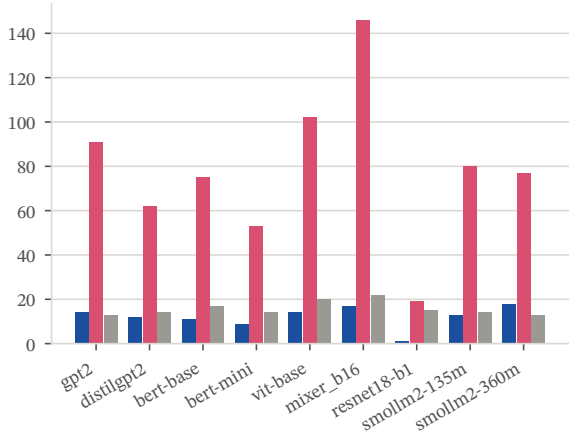
ms in the collector over the timed loop (lower is better)
