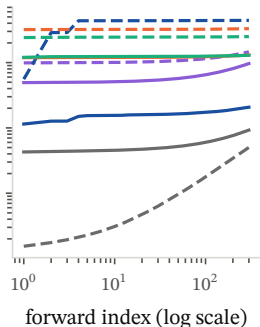
tiny-gpt2
