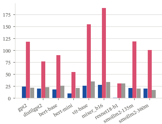
ms in the collector over the timed loop (lower is better)
