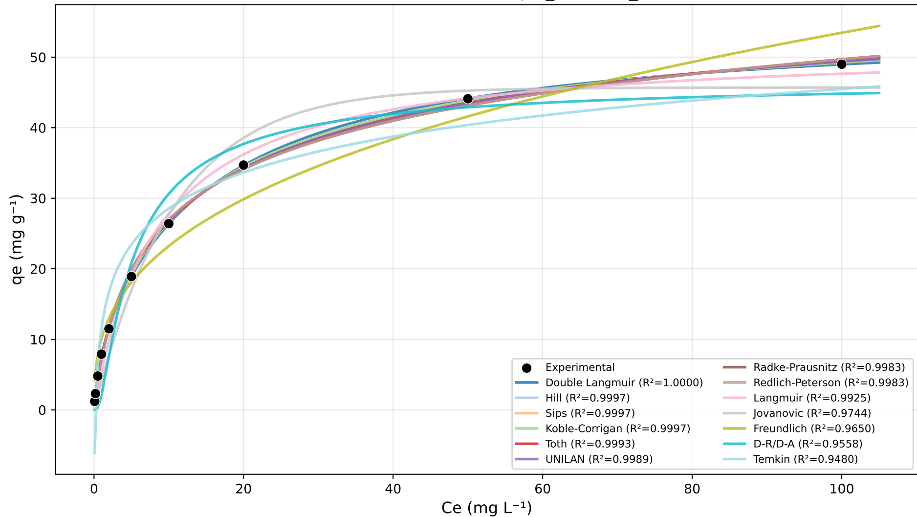
All Isotherm Model Fits — sample_isotherm_data.csv
