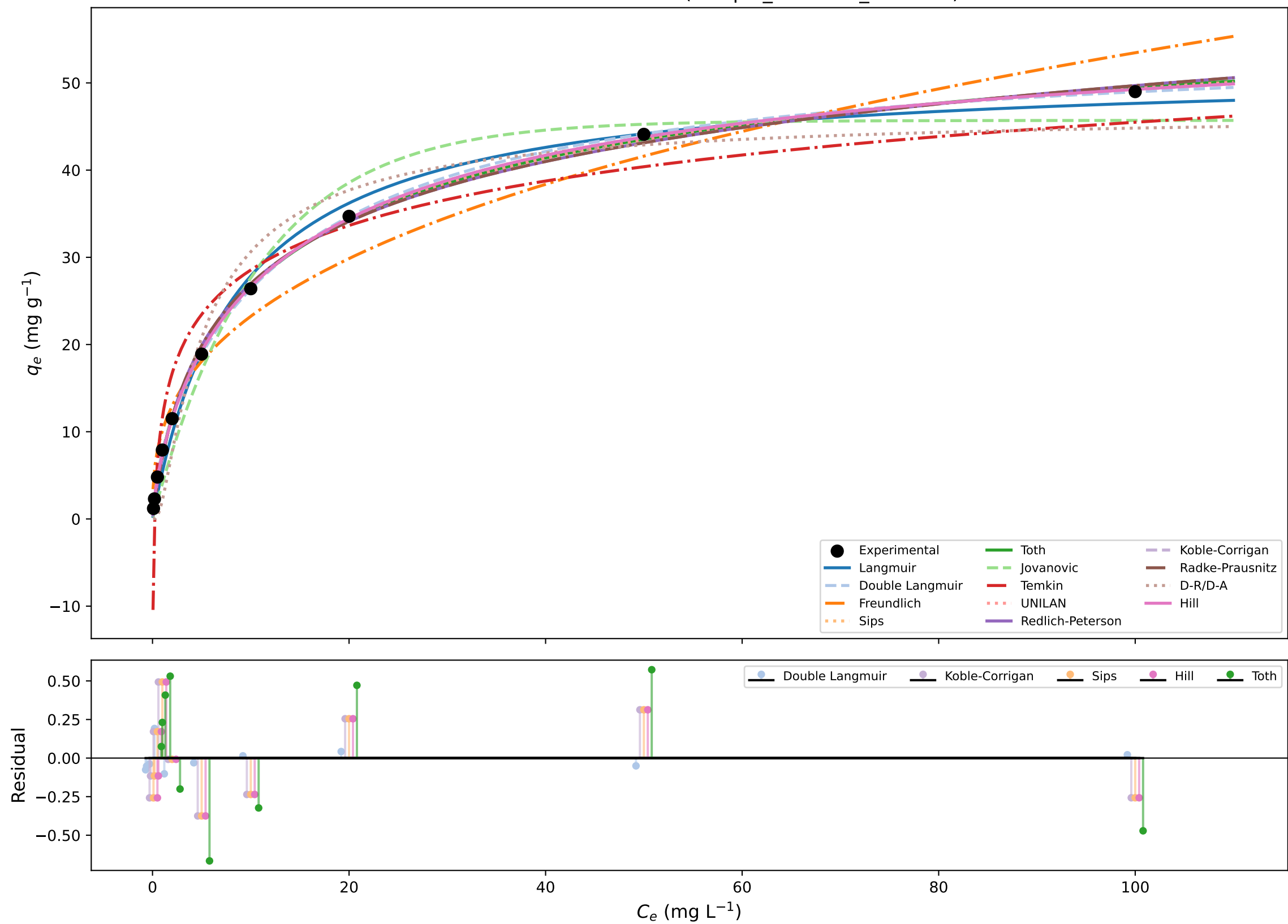
Isotherm Fits — All Models (sample_isotherm_data.csv)
