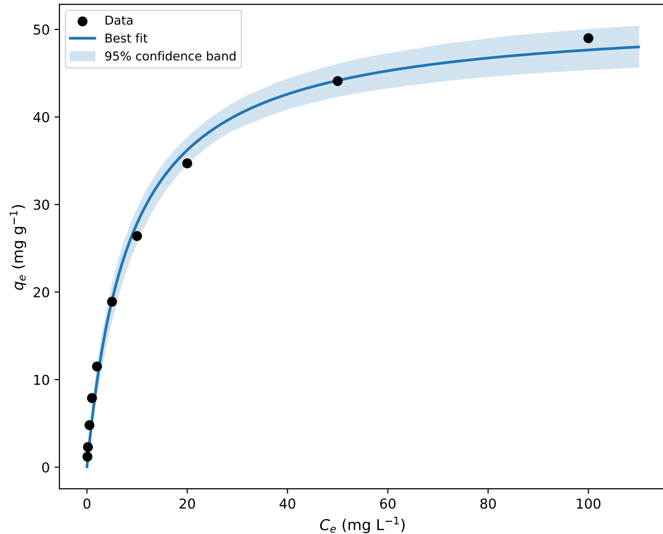
Langmuir — 95% Confidence Band
