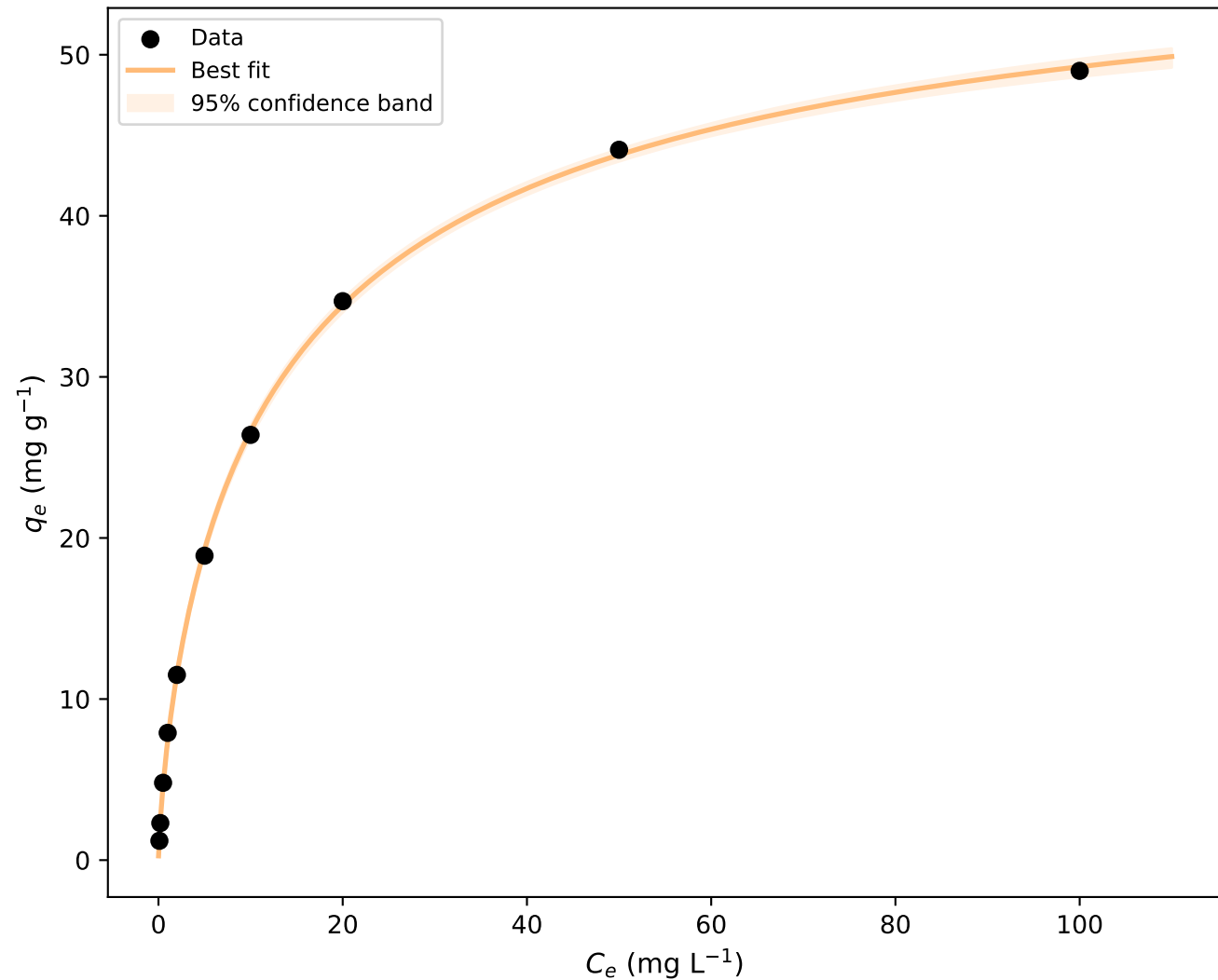
Sips — 95% Confidence Band
