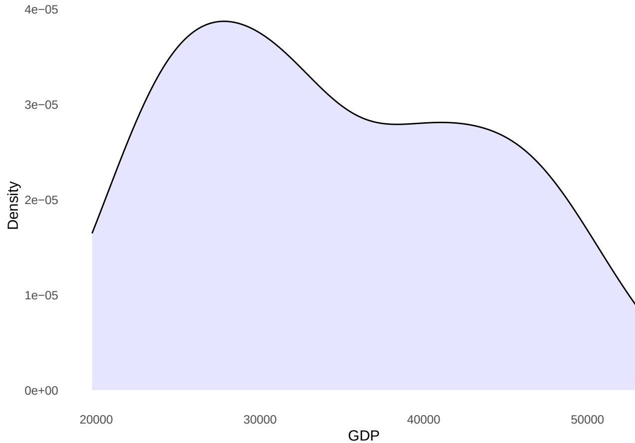
Density Plot of GDP
