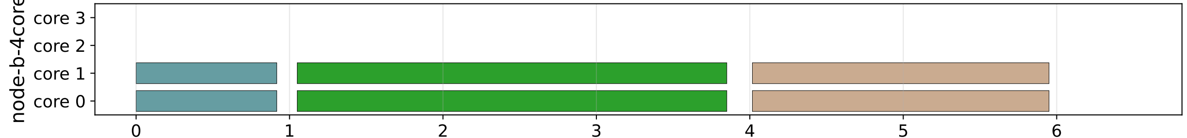
node-b-4core (n2d-highcpu-4) — job → core assignment
