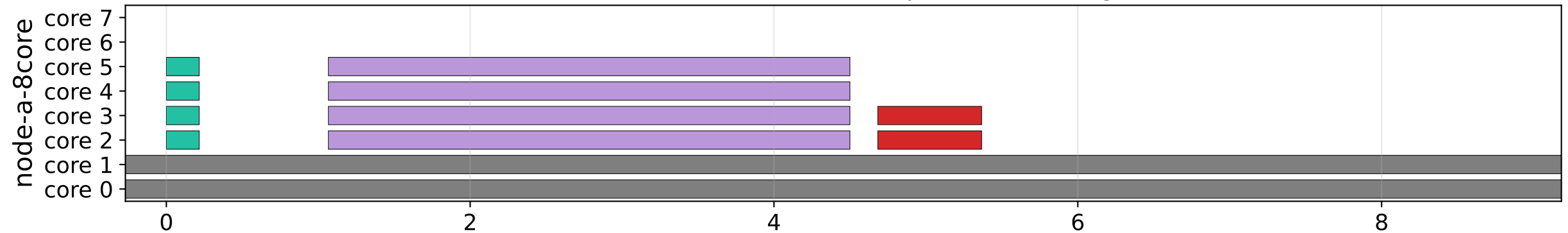
node-a-8core (e2-standard-8) — job → core assignment
