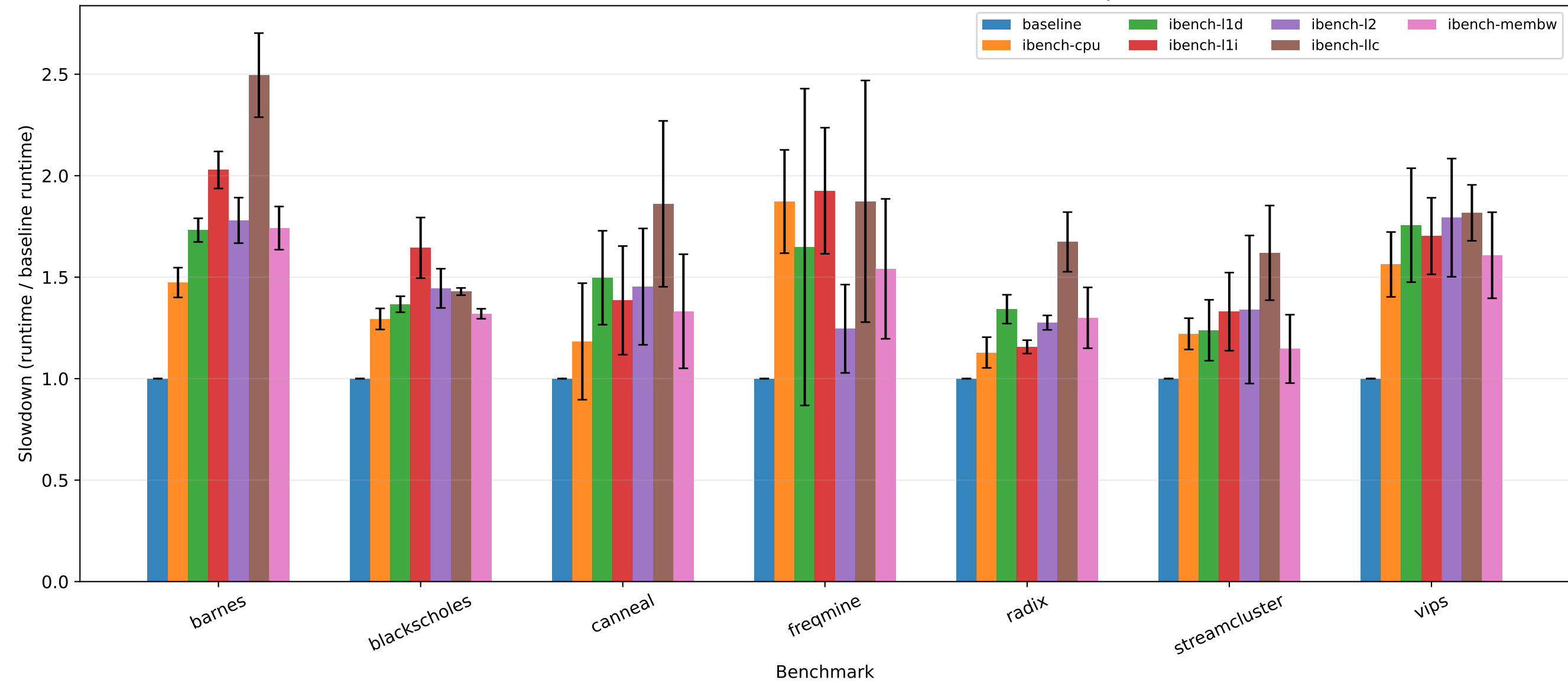
Part 2a: Runtime slowdown vs baseline (3 runs, mean +/- sample std)
