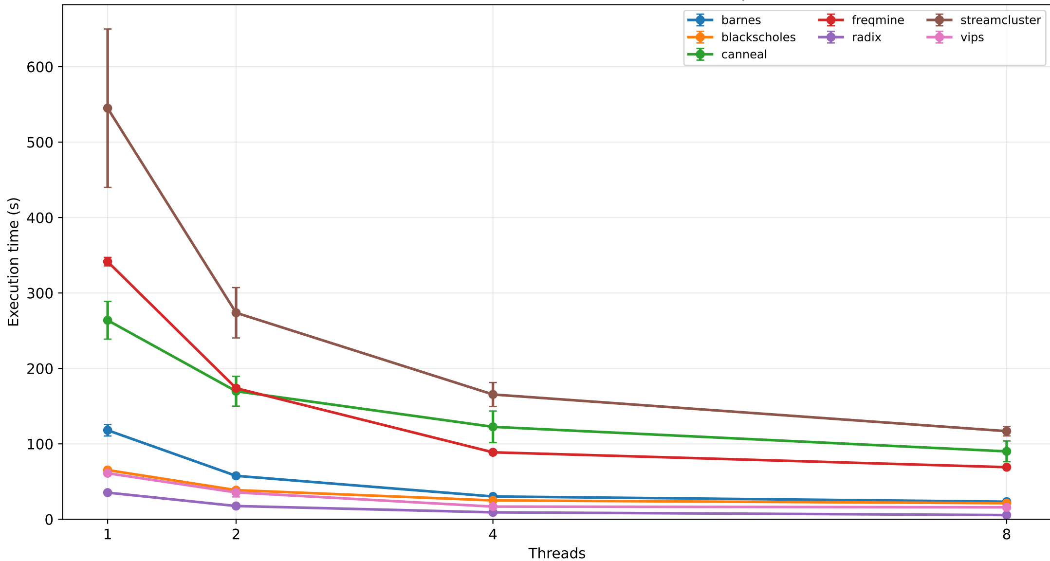
Part 2b: Runtime vs threads (3 runs, mean +/- sample std)
