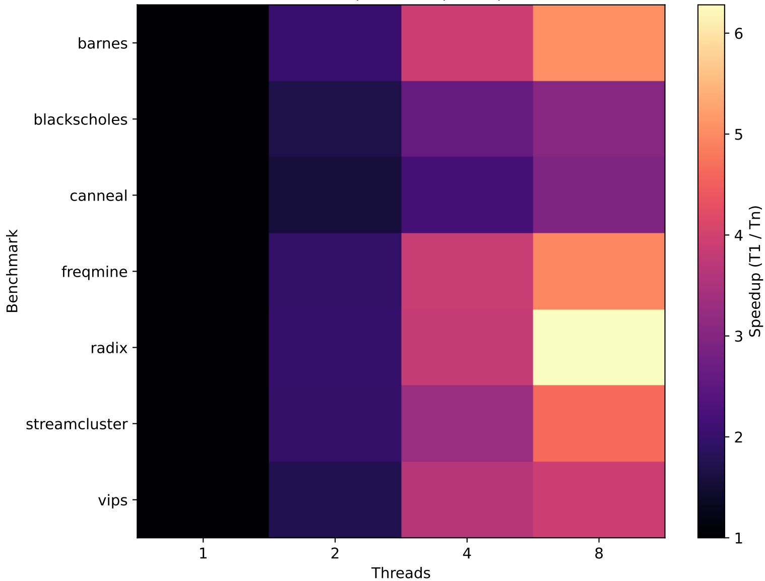
Part 2b heatmap: mean speedup (3 runs)
