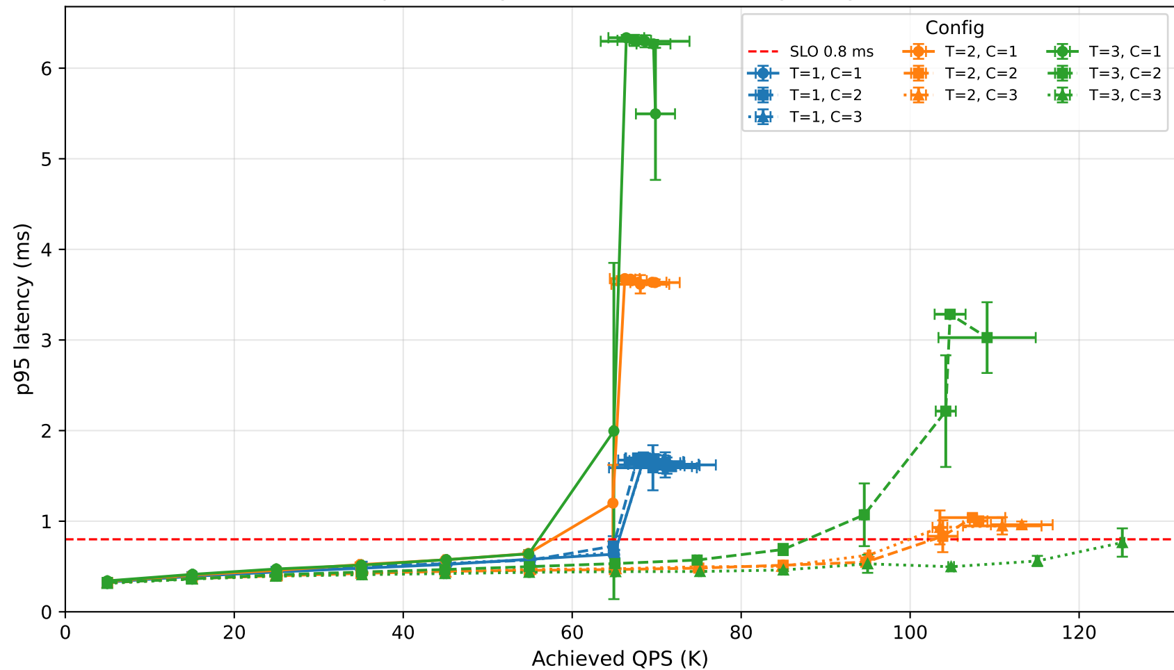
Memcached p95 latency vs QPS — all T×C configs (avg over 3 runs)
